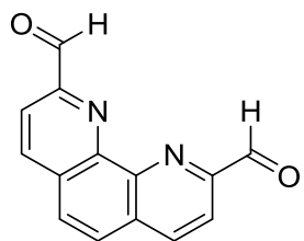
Phenanthroline ligand
