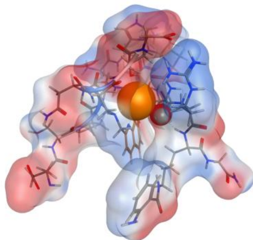
Synthetic enzyme
